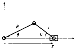
Fig. 2. Planar RRRP mechanism.
