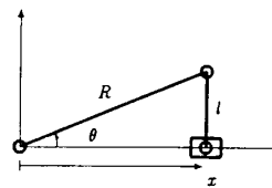
Fig. 3. Second kind of singularity for the planar RRRP mechanism.
