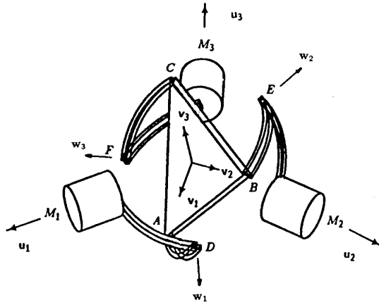
Fig. 9. Spherical three-degree-of-freedom parallel manipulator.
